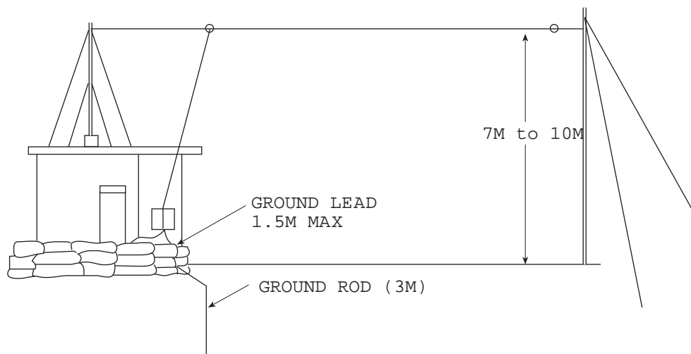
BASE INSTALLATION
